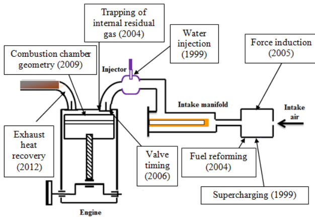
Fig. 2 Literature on HCCI engine fuelled with ethanol.
